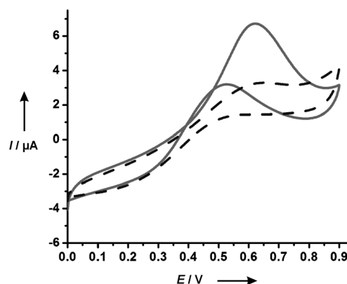
Figure 2. Cyclic voltammograms of hollow spherical CoPt nanoparticle superstructures (solid line) and CoPt nanoparticles (dashed line) in \text{H}_2\text{SO}_4 (0.5 M) containing methanol (0.6 M). Note: sweep rate = 0.05 \text{ V s}^{-1} ; loading \approx 7.5 \mu\text{g} .
