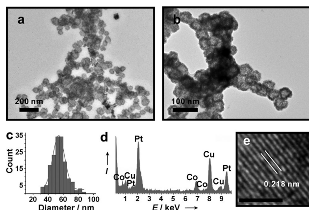
Figure 1. a, b) TEM images of hollow spherical CoPt nanoparticle superstructures. c) Diameter distribution of CoPt nanoparticle superstructures ((53.9 \pm 7.9) \text{ nm}) ; based on 158 counts). d) EDS data for CoPt nanoparticle superstructures (Cu is from the TEM grid). e) HRTEM of a single CoPt nanoparticle showing the lattice fringes (scale bar: 2 nm).
